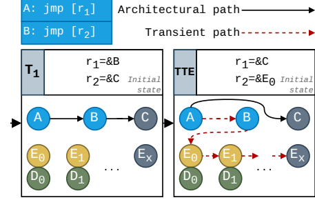
Figure 1: Injecting RSB entries in the transient execution window of an indirect branch (TTE BT-RSB ). In T_1 , A is trained to execute B . Next, in TTE , A transiently executes B , which in turn executes a series of call gadgets E_i , each followed by a disclosure gadget D_i .
